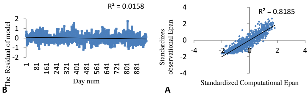
Fig. 4- Distribution diagram and residues of Bayesian model of Jolfa station
