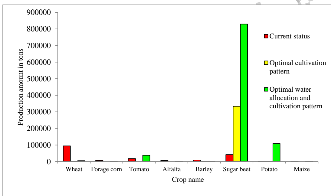
Fig 2- Comparing the amount of product production in the current situation with optimization models
